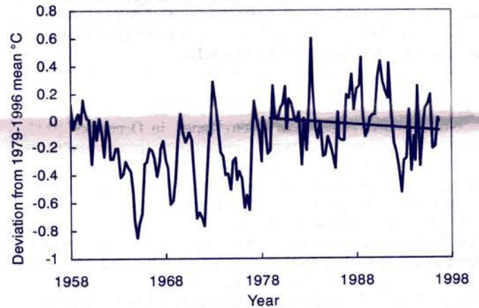
Fig. 5. Radiosonde balloon station measurements of global lower tropospheric temperatures at 63 stations between latitudes 90 N and 90 S from 1958 to 1996 (15). Temperatures are three-month averages and are graphed as deviations from the mean temperature for 1979 to 1996. Linear trend line for 1979 to 1996 is shown. The slope is minus 0.060 °C per decade.
